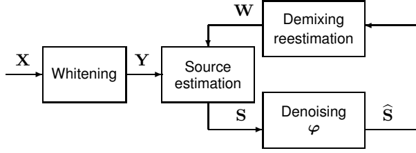
Figure 1: The general iterative procedure of the algorithmic framework of DSS.
