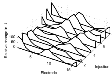
Figure 2. Relative changes in potentials compared to homogeneous background. The eight curves correspond to injections from eight different electrodes.
