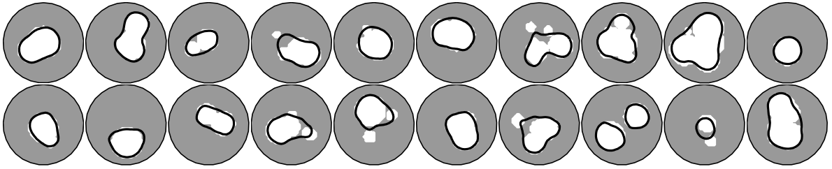
Figure 3. Examples of bubble formations reconstructed with Bayesian MLP. The white blobs show the actual simulated bubbles and the black lines show the contours of the reconstructed bubbles.
