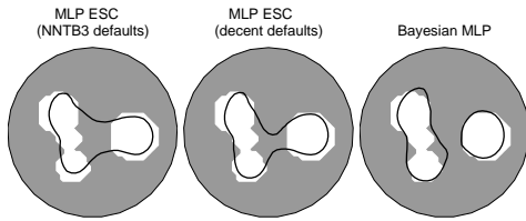
Figure 4. Example of the image reconstruction with Bayesian MLP and early stopping committees. See text for explanation of the models.
